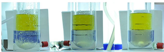
Figure 3. Gasoline/water phases of QWT samples at three pHs after demixing experiments; pH 5 (left), pH 7 (middle) and pH 9 (right). Turbidities of 3, 10 and 197 NTU, respectively.
