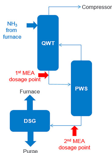
Figure 4. Representation of the process water section from a liquid cracker with MEA dosing points.
