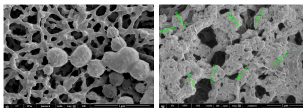
Figure 2. Scanning electron microscopy (SEM) images of cellulose nitrate filter; unused filter (left) and filter after filtration of liquid cracker PW (right).
