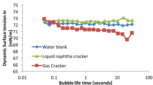
Figure 1. Dynamic surface tension measurements can determine the presence of surface active agents.
