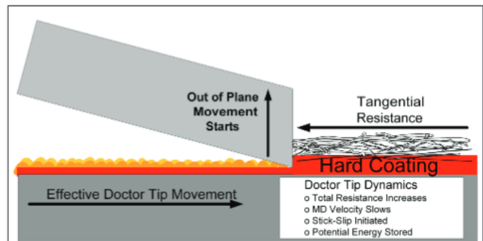
Figure 6a - High resistance to MD movement encountered
