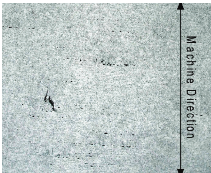
Figure 1 - Sheet chatter
