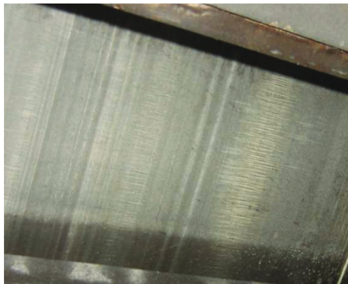
Figure 2a - Bands of coating chatter
