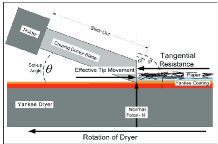
Figure 5 - The system of interest when defining chatter
