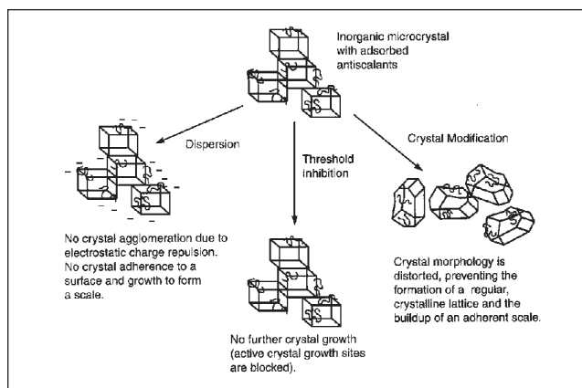
Figure 2 — Primary chemical scale control mechanisms: dispersion, threshold inhibition and crystal modification
