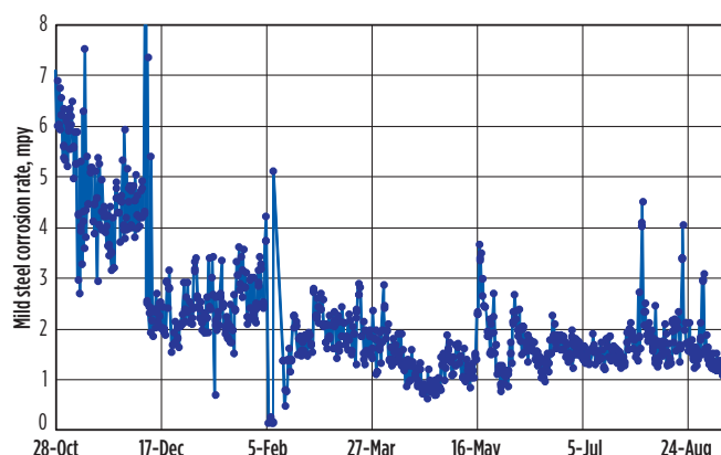
FIG. 2. Mild steel corrosion rate improvement with new program, with a target of < 4 mpy.
