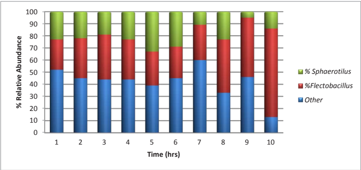
Figure 6: Relative abundance of Sphaerotilus and Flectobacillus genera in the effluent biofilm over time.
