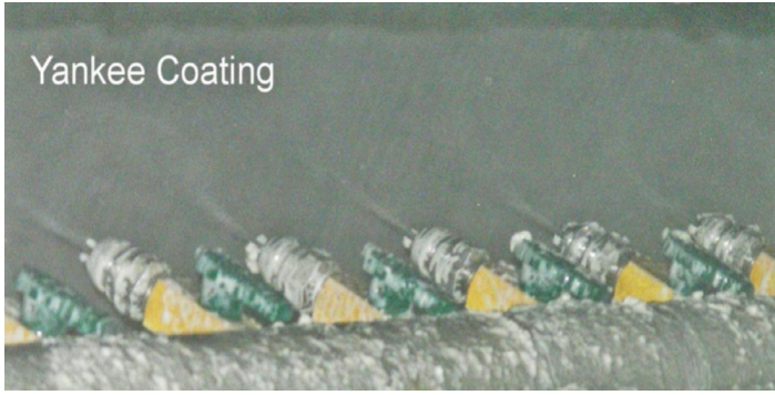
Figure 1 - Photograph showing a functional coating on a Yankee dryer that is uniform.
