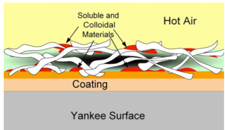
Figure 8 - Illustration showing that ultimately some of the materials on the surface of the fibers become part of the coating and affect its characteristics.
