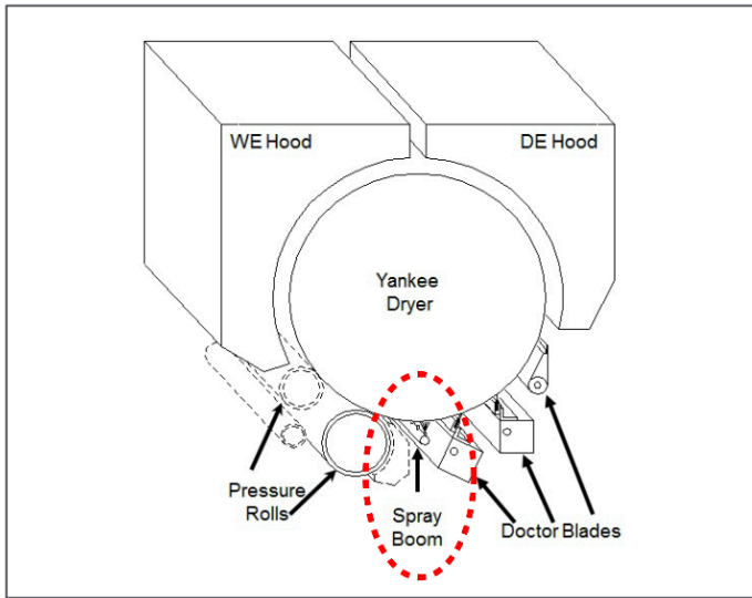
Figure 9 – Indicates the location of the spray boom utilized to apply unique coating materials to the Yankee dryer.
