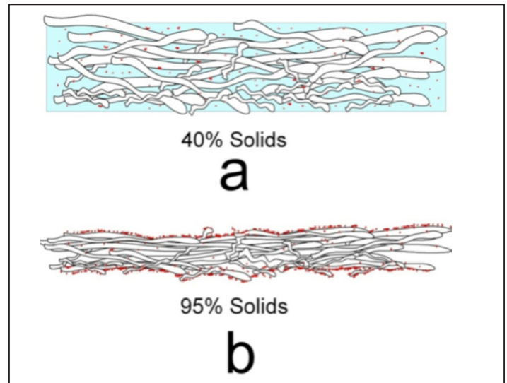
Figure 7 - Illustrations demonstrating the Dreshfield effect. (7a) As the sheet leaves the pressure roll nip at 40% solids, some chemicals along with fines and colloidal materials are dispersed in the free water between the fibers. (7b) As the sheet dries, the smaller materials concentrate as they move to the surfaces of the sheet.
