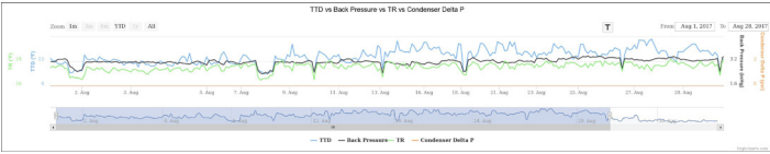
Figure 2: High Backpressure and Terminal Temperature Difference (TTD) with normal Delta P and Temperature Rise (TR) indicate an air leak. The data confirmed the diagnosis.
