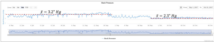
Figure 4: Backpressure decreased from 3.2" Hg to 2.3" Hg, an improvement of 0.9" Hg and an efficiency gain of 0.9%
