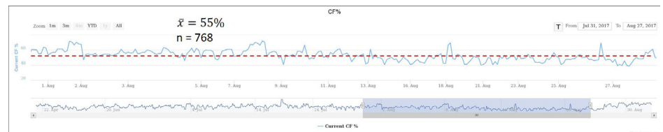
Figure 1: The average cleanliness factor of 55% for August was well below the design
