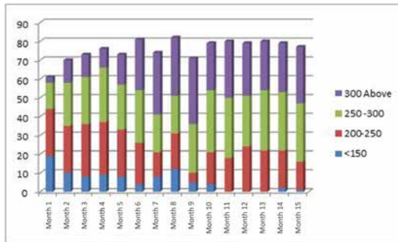
Figure 1 - The bladder curing frequency is improved after 3D TRASAR Boiler Technology was applied.
