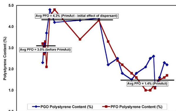
FIGURE 3: POLYSTYRENE LEVELS DECREASE WITH NALCO WATER PRIMACT
