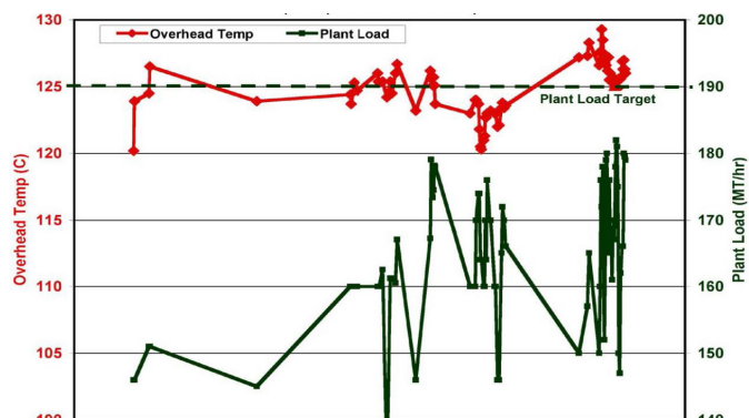
FIGURE 4: CURRENT THROUGHPUT EXCEEDS PREVIOUS LEVELS WITH NALCO WATER PRIMACT
