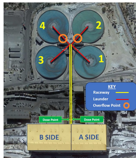
FIGURE 1: Site setup and Nalco Water dosage points for the tailings launder solution.
