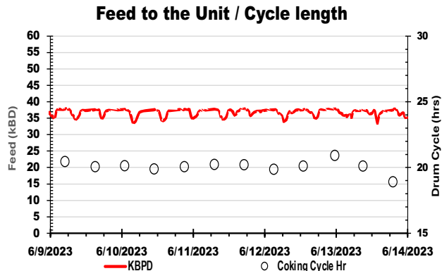
Fig. 1: Performance with the old coker antifoam
