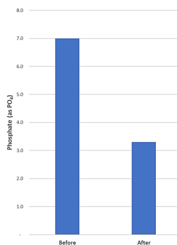
Figure 2: Changing to the low-phosphorus program reduced phosphate concentrations in the recirculating water by 53%
