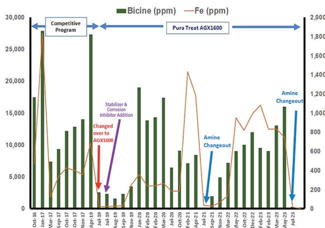
Figure 1: Bicine levels of amine system pre and post program change.
