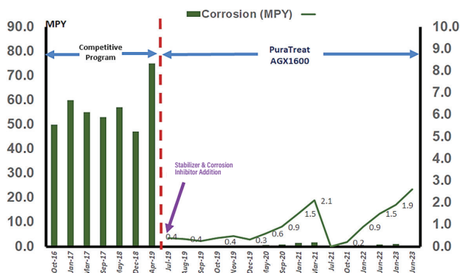
Figure 2: Corrosion levels of amine system pre and post program change.
