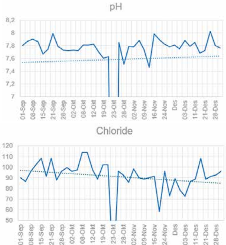
Figure 2. pH and chloride profile of cooling water during non-phosphate trial.
