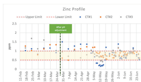
Figure 1.b Zinc level could be maintained below <1.0 ppm at least 80% during the trial period after maintaining pH 8 - 8.5. Non-P corrosion inhibitor program reduced the consumption of Zn program, 3DT129, because of lower phosphate level. The program was further optimized after trial.
