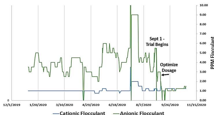
FIGURE 1. Polymer Optimization with the ADPAS Liquid System
