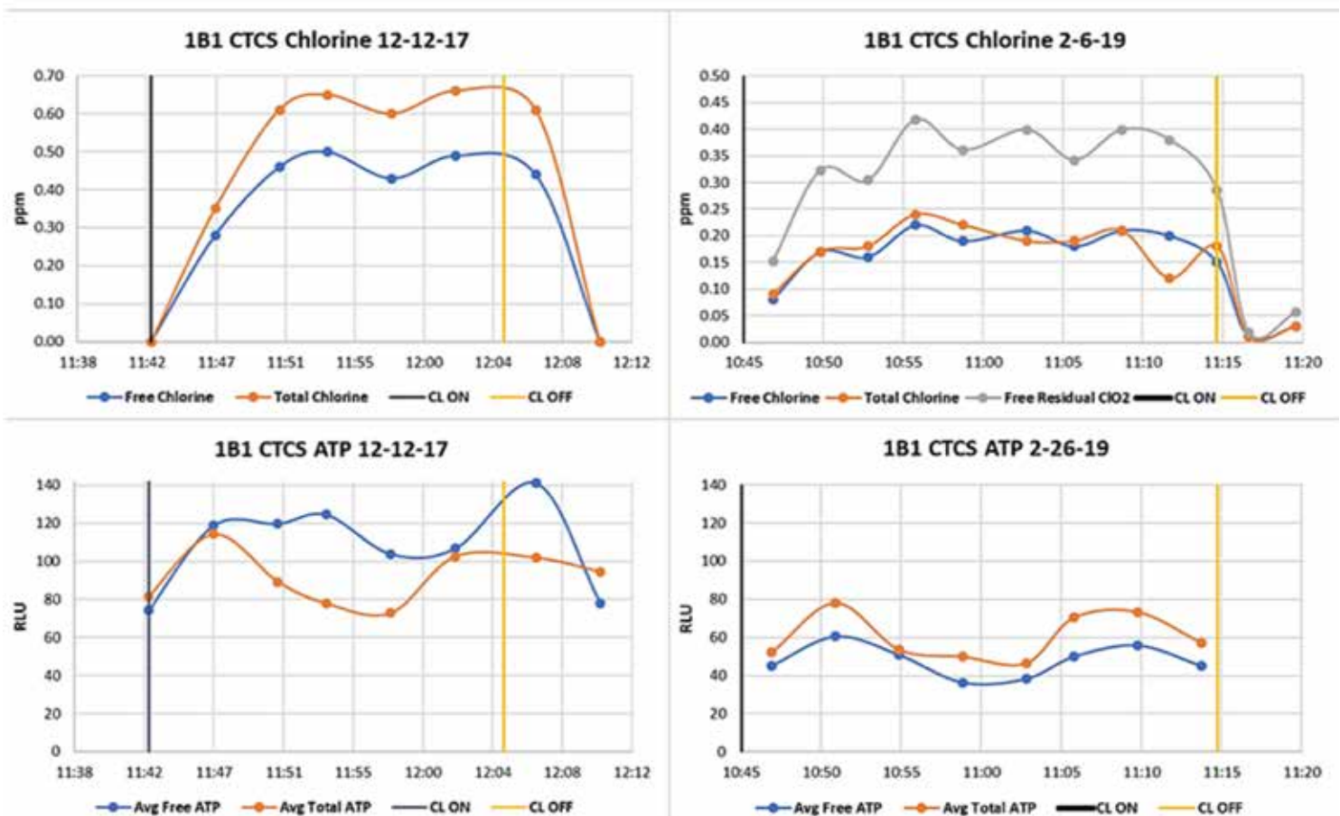
Figure 1: Performance comparison between bleach and chlorine dioxide
