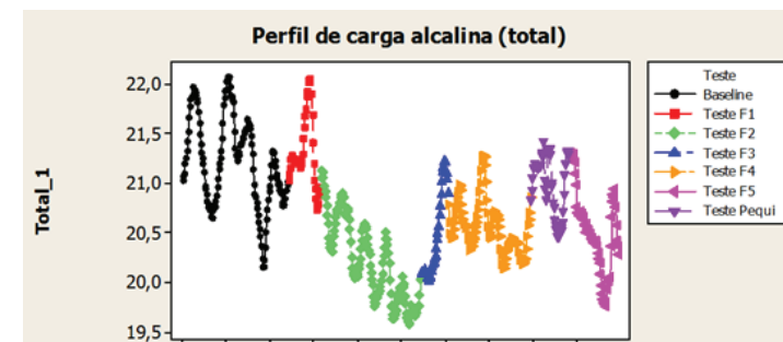
Figure 1. Reduced alkali charge per ton of wood produced
