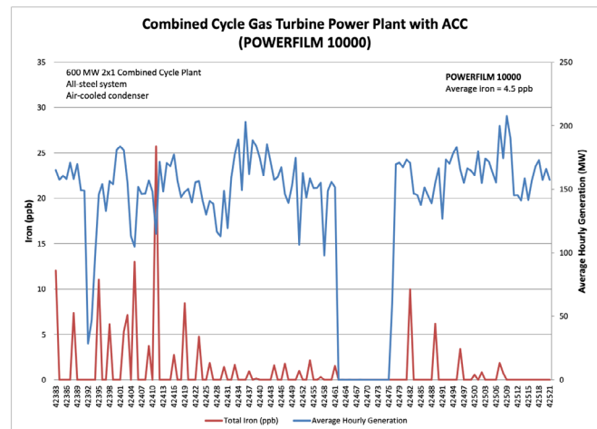
Figure 2: Operational graph showing corrosion product reduction using Nalco Water POWERFILM™ 10000
