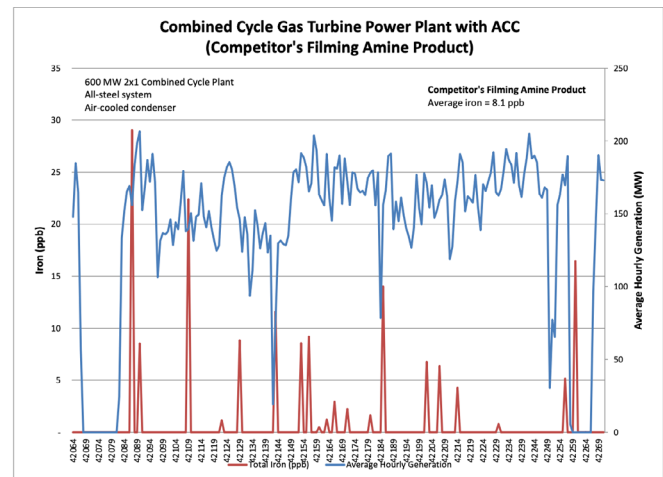
Figure 1: Operational graph showing corrosion product generation under competitor's filming amine product.
