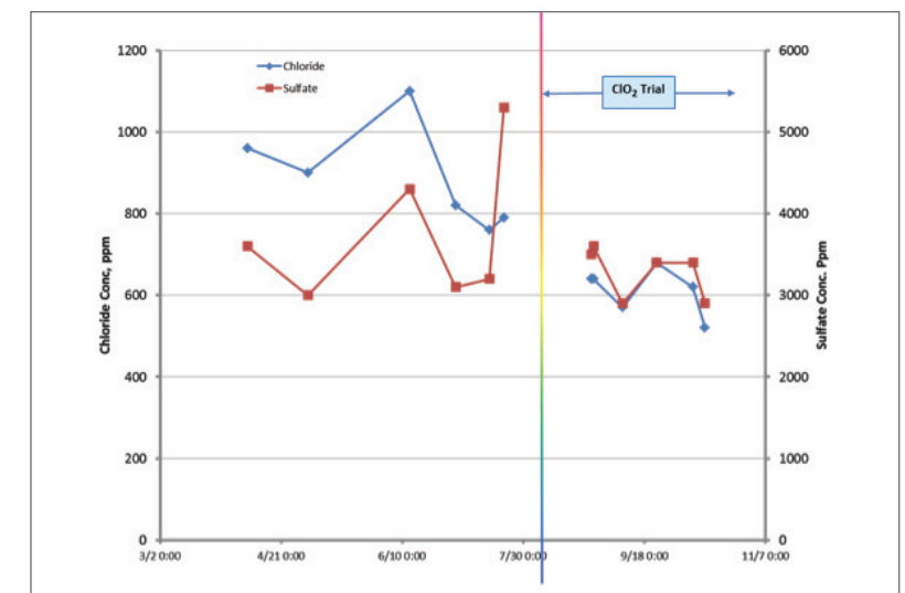
Figure 6 - Cooling water sulfate and chloride levels
