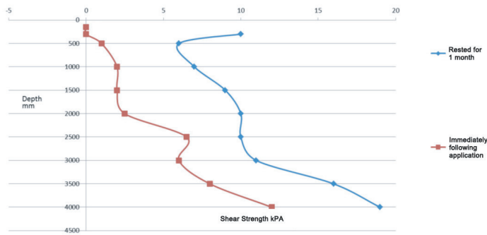
Figure 3 - OreBind Rheology Improvements in a Tailings Storage Facility
