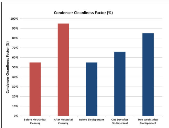
Figure 3 - Cleanliness Factor showed the same trend as condenser backpressure. Mechanical cleaning and biodispersant delivered almost equivalent results without the availability loss associated with an outage.
