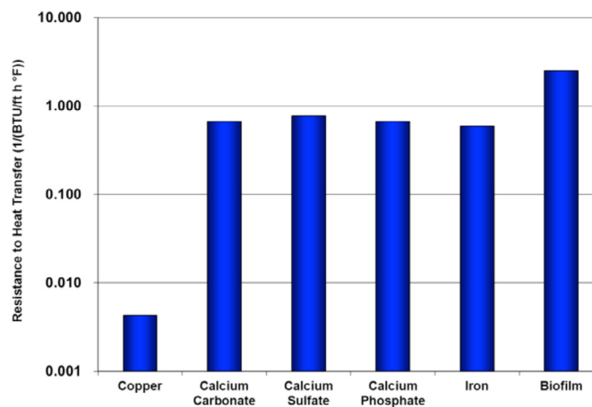
Figure 1 – Biofilm has a higher resistance to heat transfer than other deposits. Note also the impact of deposition on heat transfer when compared to other deposits and copper, the material of construction of many heat exchangers.
