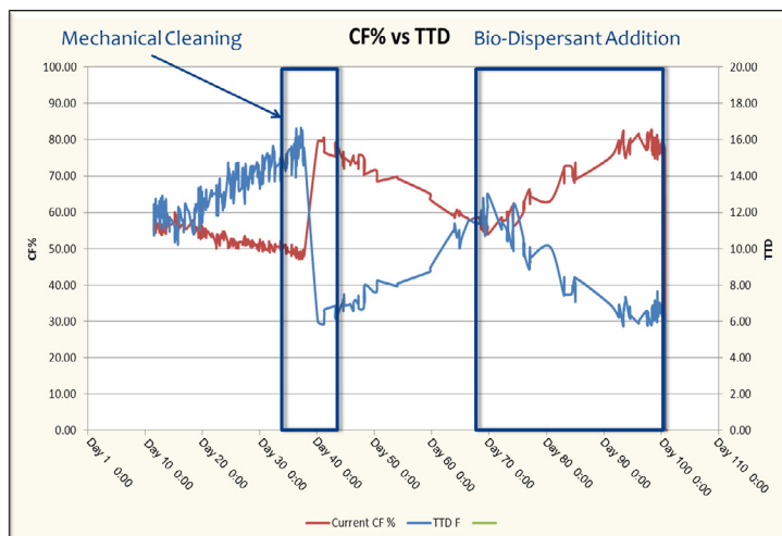
Figure 4 - The comparative effects of the mechanical cleaning and bio-dispersant application are shown in this graph from the plant's DCS.
