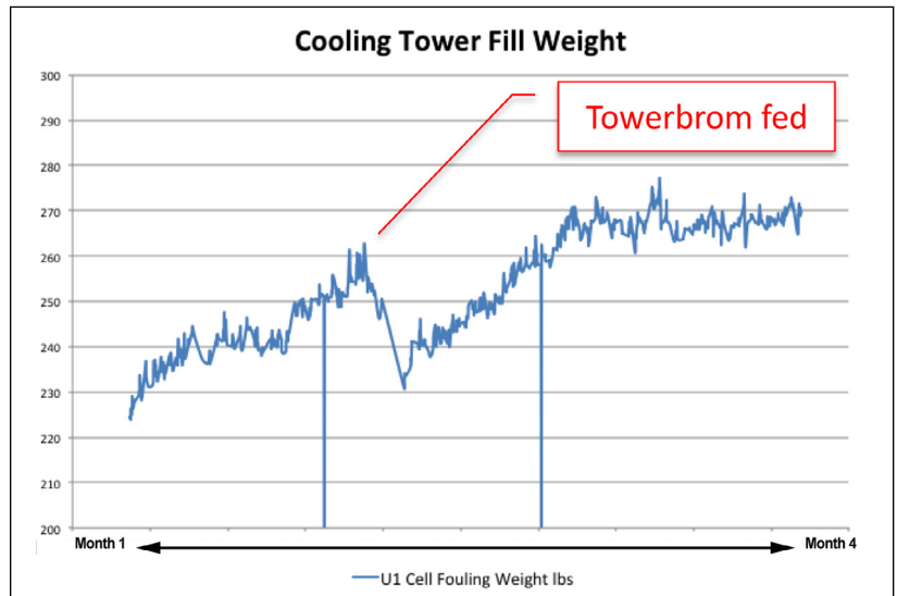
Figure 4 - The actual cause of the problem was microbial fouling in the cooling tower. When the deposits were removed, the weight of the cooling tower fill dropped. When the biodispersant program was discontinued, the weight increased again.
