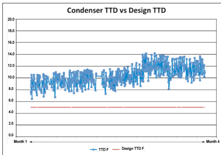
Figure 3 - Condenser Approach Temperature -- or Terminal Temperature Difference (TTD) also rose during this period, leading to the initial diagnosis of a fouled condenser.
