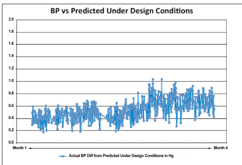
Figure 2 - Condenser Backpressure increased.
