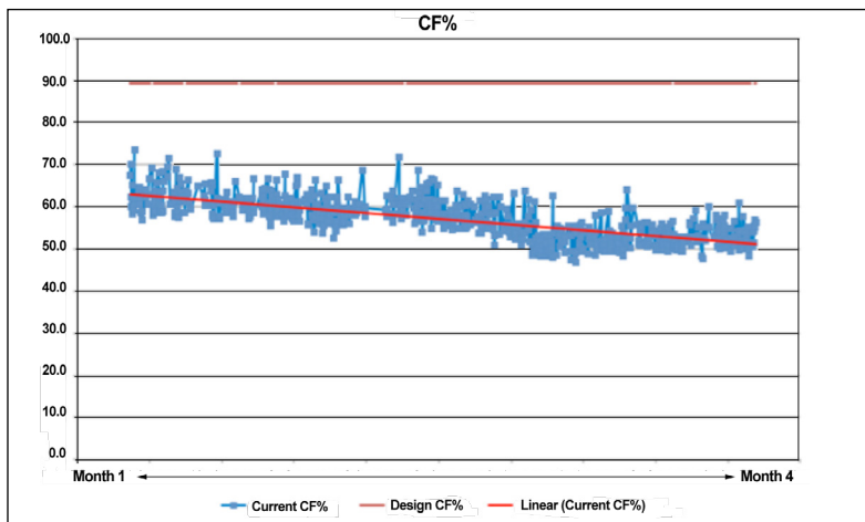
Figure 1 - Cleanliness Factor decreased.
