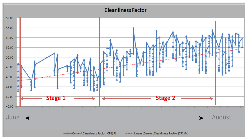
Figure 5 - Cleanliness Factor across the entire evaluation period
