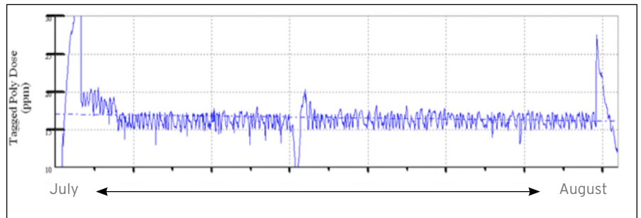
Figure 4 - Dispersant polymer use was high during the first 5 days of Stage 2 and then leveled off as demand subsided.
