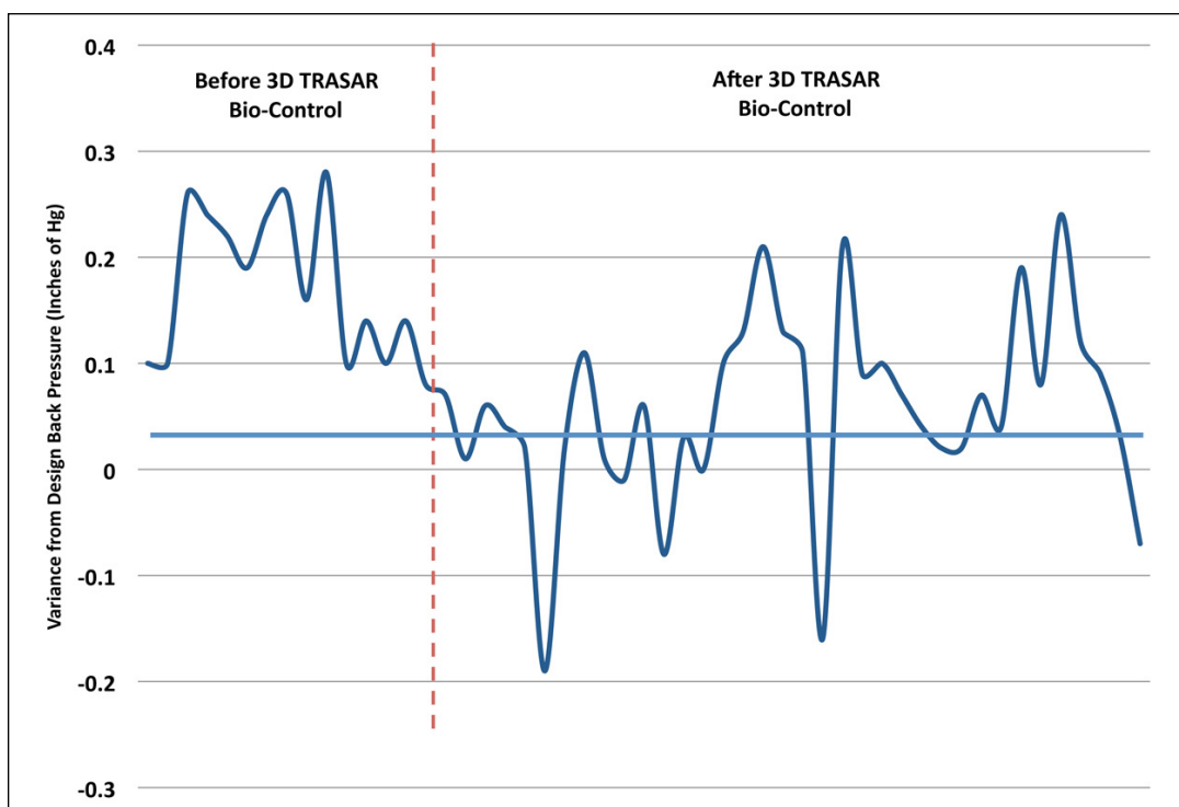
Figure 3 - Variance from Design Back Pressure is the difference between the measured back pressure and the design back pressure. There was no measurable change in performance after implementation of 3D TRASAR Bio-Control, indicating that better control of the oxidant delivered equivalent results at a lower oxidant concentration.
