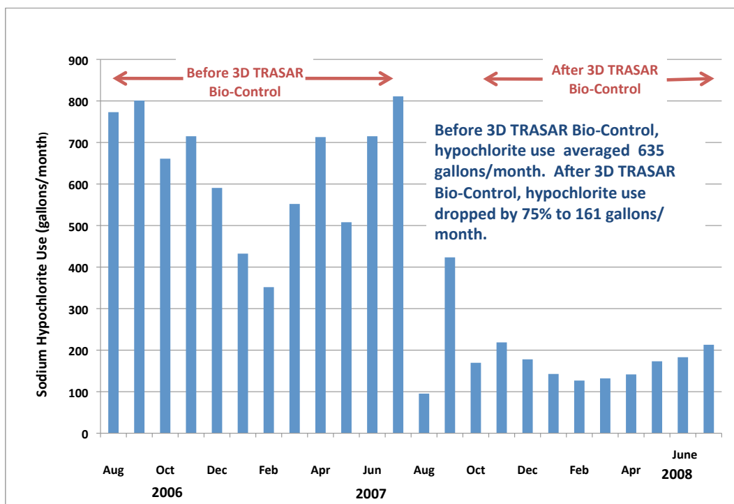
Figure 2 - 3D TRASAR Bio-Control delivered equivalent microbial control, but required 75% less oxidant.
