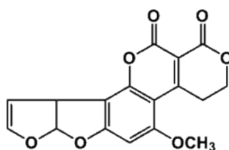
Aflatoxin G 1
