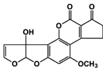
Aflatoxin M 1
