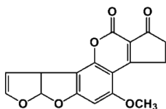
Aflatoxin B 1
